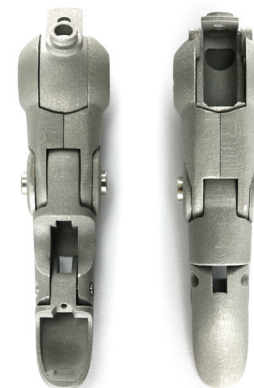
Prosthetic Finger Assembly
