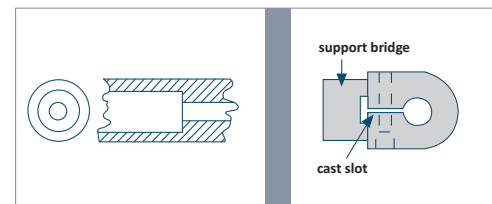
Examples of support using a counter bore
